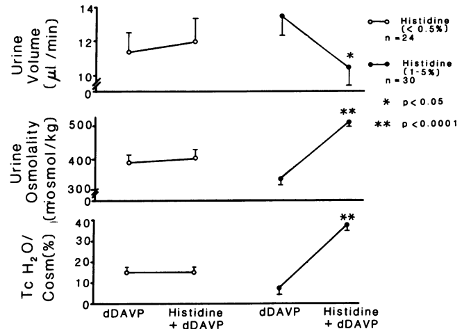
Figure 3. The effects of low doses of histidine (0–0.5%) are compared with those of high dietary histidine (1–5%). (○) Low-dose histidine; (●) high-dose histidine. High doses of histidine have a profound effect on the concentrating ability. This is quite different from the lack of effectiveness shown for the low-dose histidine group. Note that histidine concentration in this and subsequent figures represent percent histidine by weight added to the regular laboratory diet that contained 0.51% histidine.
