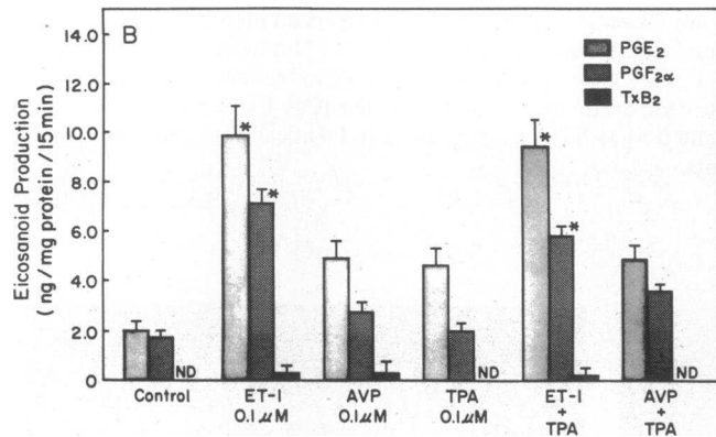
Figure 4. Release of [ 3 H]arachidonate and synthesis of immunoreactive arachidonate metabolites in response to ET-1 and AVP. (A) Mesangial cells at 80% confluency in six-well plates were equilibrium-labeled for 20 h with 1 μCi/ml [ 3 H]arachidonate. After washing the cells, agonists were added and release of radioactivity into HBSS-II was measured at the times indicated as described in Methods. Data are mean ± SEM for three experiments in duplicate. (B) Mesangial cells at 80% confluency in 12-well plates were incubated with the effectors indicated for 15 min at 37°C in RPMI 1640 medium in 5% CO 2 /95% air. Release of immunoreactive PGE 2 , PGF 2α , and TXB 2 into the supernate was quantified by RIA. Data are mean ± SEM for four to five experiments in duplicate. *Significantly different from control values ( P < 0.05 ) by Student's t test. ND, not detectable with a minimum detectable limit of 0.05 ng TXB 2 /mg protein per 15 min.
